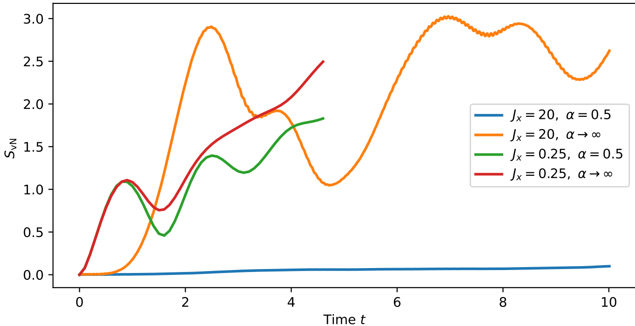
N = 16 , half-chain entanglement entropy for entangled state (2,14;3,14)
